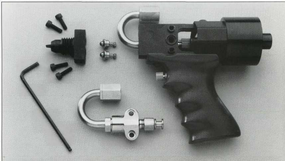
NO-PURGE SNUFF-BACK STATIONARY MOUNTING
