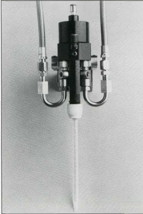
NO-PURGE SNUFF-BACK STATIONARY MOUNTING
